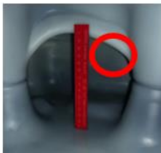
Figure 2: NG fuel tank. Allows for stuck sensor condition.
