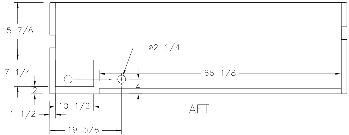
VTDP & NSDP FORWARD PANEL VIEW FROM TOP
