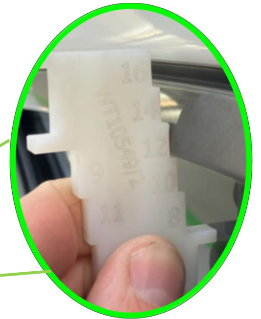
Record measurement (Profile Tool WT10549/2)
