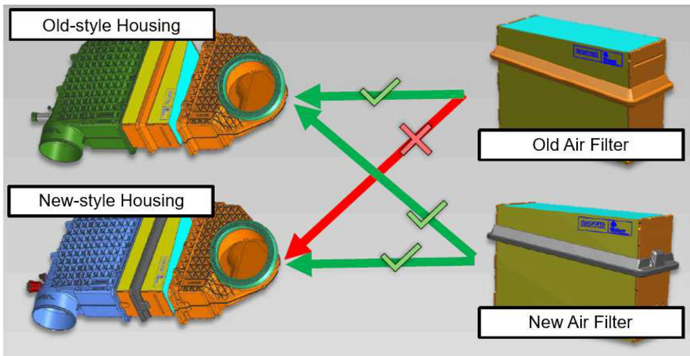
Air filter compatibility: P621725 and P621730 (top right), P640016 and P640017 (bottom right)
