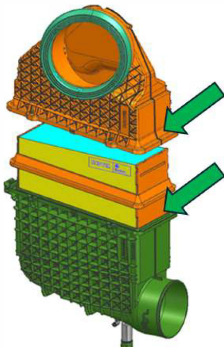
Old-style air filter housing (without tab)
