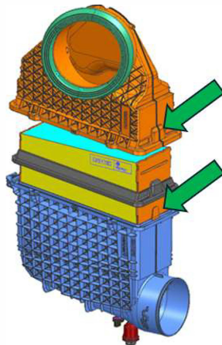
New-style air filter housing (with tab)
