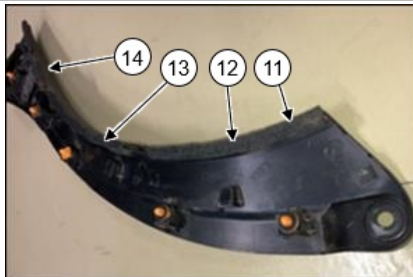
Urethane Pads (11-14) attachment completed (on rear door fender arch garnish)
