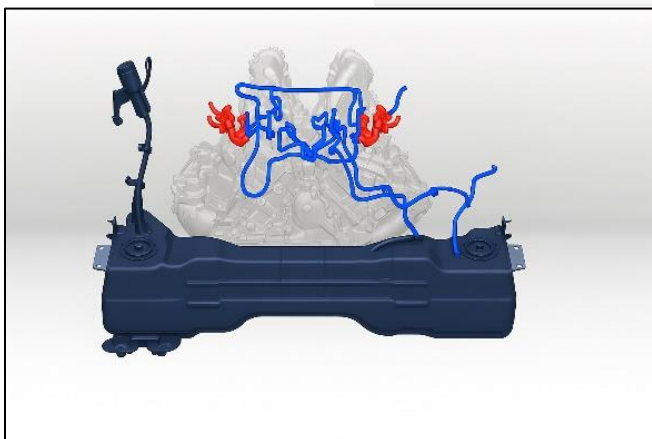
MC20 Fuel Tank
