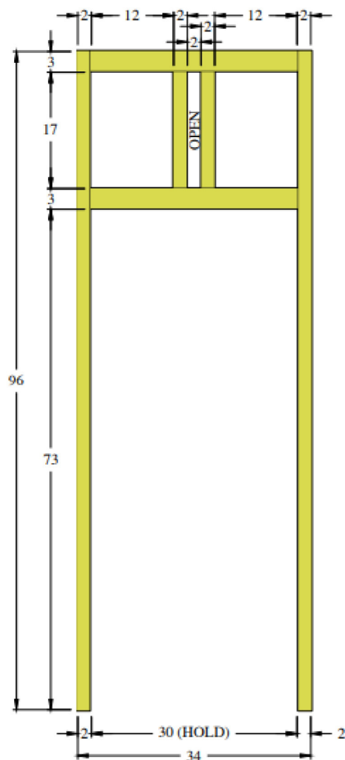
FACE A Viewed From Back Side
