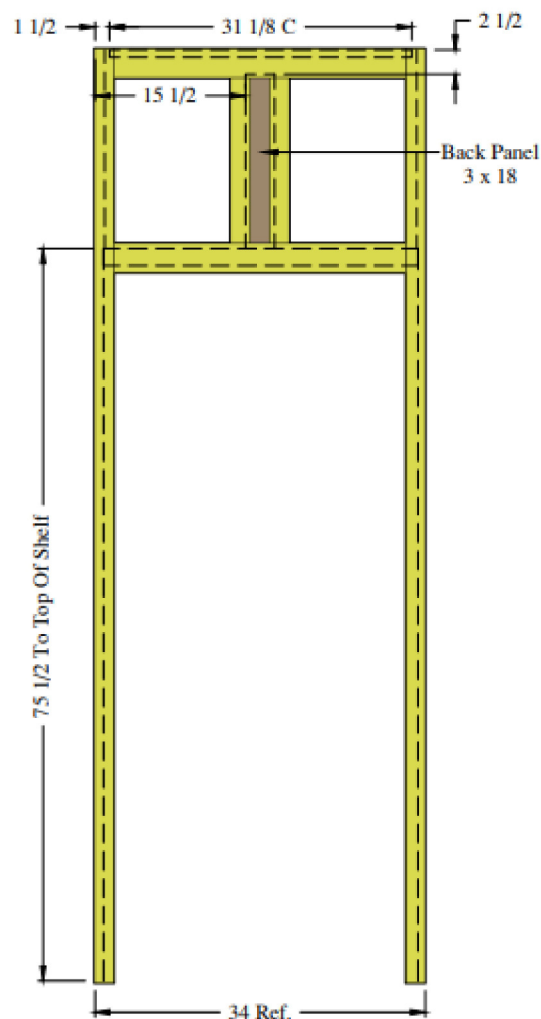
FACE A - Cleat Locations Viewed From Front Side
