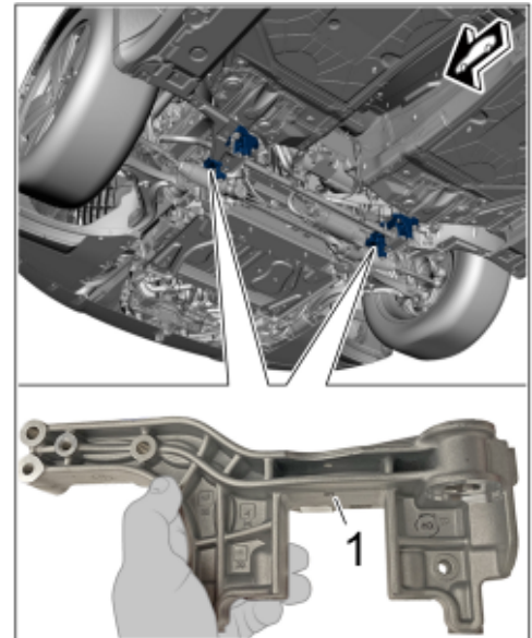
Replace anti-roll bar fastening
