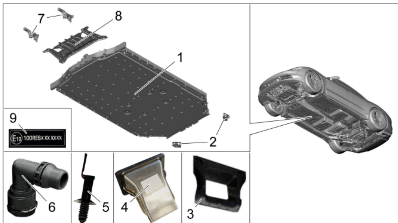
Component overview
