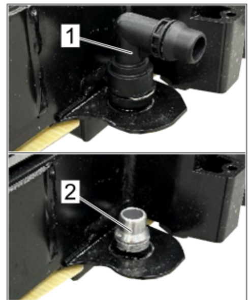
Install coolant nozzles
