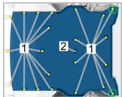
Screw points for front cover
