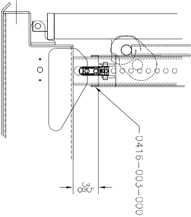
WELD FLAT BAR TO LIMIT DECK BOTTOM POSITION
