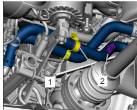
Coolant hose bracket
