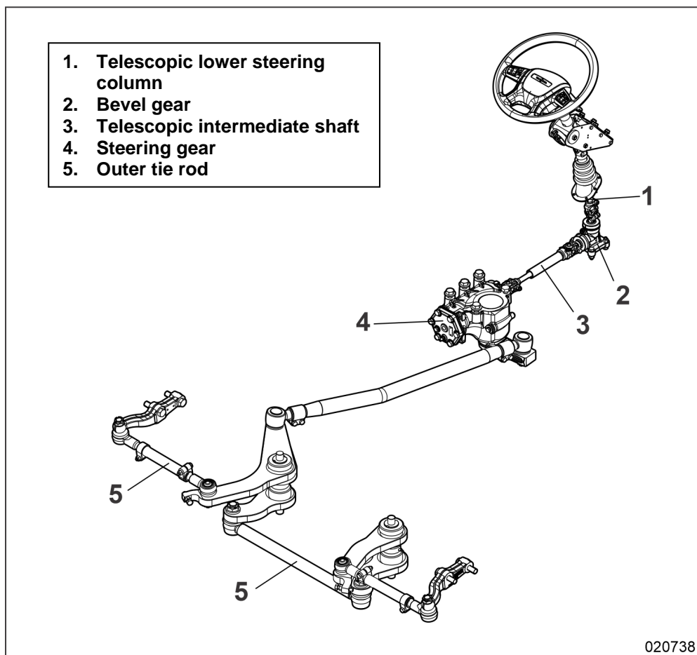
Figure 1: Front axle steering linkage
