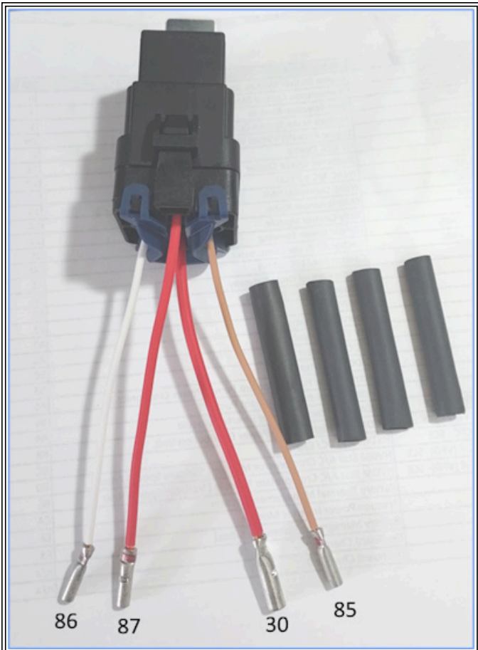
Figure 1 : Relay Kit
