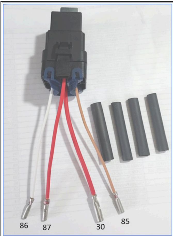
Figure 1 : Relay Kit
