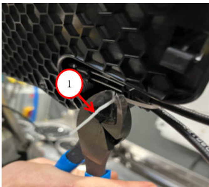
Fig. 3 Remove Excess Tie Strap End
