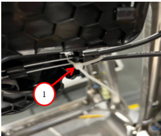
Fig. 2 Tie Strap Attached
