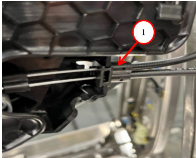
Fig. 1 Easy Entry Cable Connection
