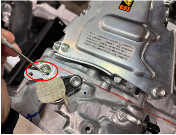
Original Design (Transmission Hole Drilled) (H3T shown, PHEV similar)
