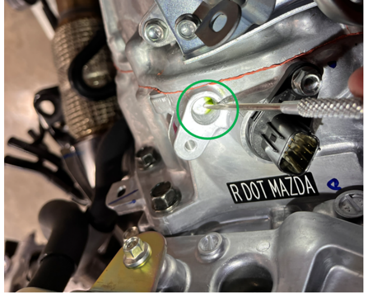
New Superseded Design (Hole Blocked) (H3T shown, PHEV similar)
