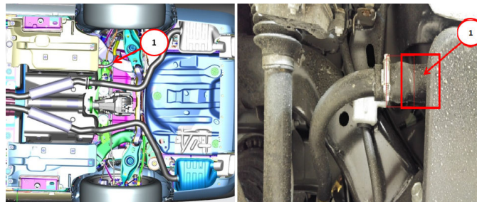
Fig. 1 Fuel Leak Inspection Area
