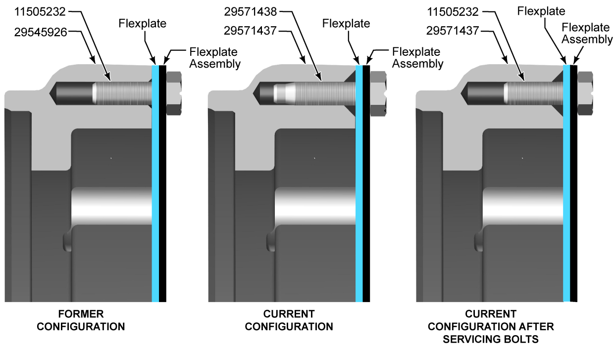
Figure 2. Acceptable Configurations
