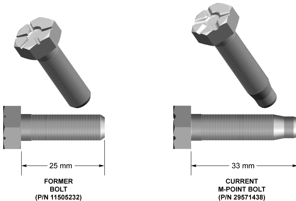
Figure 1. Flexplate Adapter Bolt Comparison
