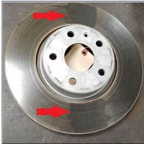
Figure 2: Brake pad imprint.
