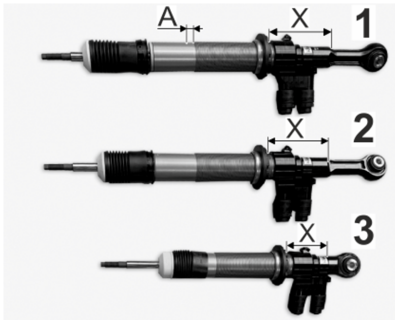
Front and rear axle spring struts adjustment dimensions
