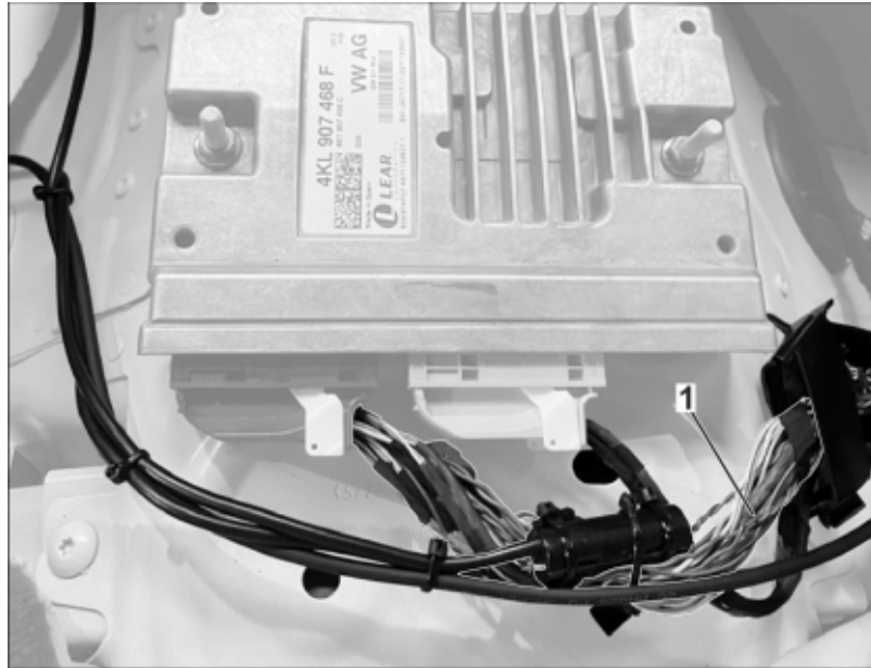
Can Clip assembly
