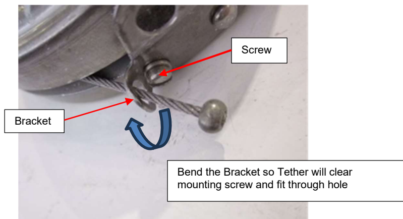
Figure 9: Tether Bracket Detail
