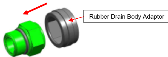
Figure 5: Installing Rubber Drain Body Adaptor over Cartridge Hex Fitting
