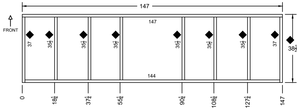
DINETTE SLIDE ROOF
