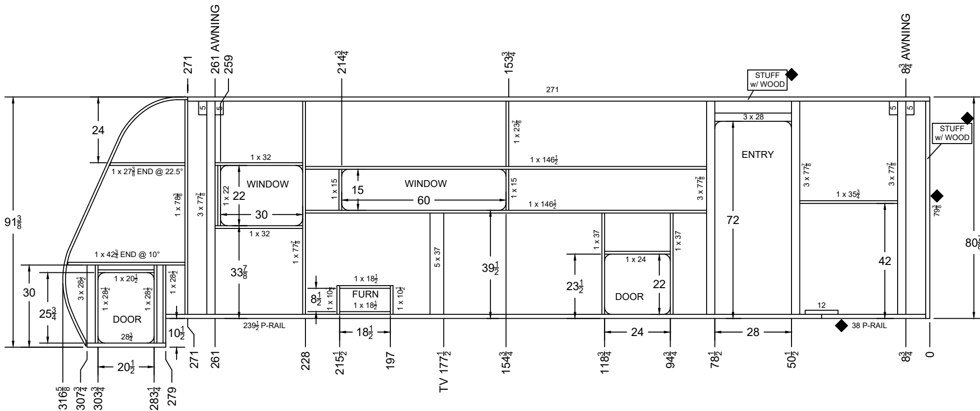
AL2600 DS SIDEWALL CUT LIST
