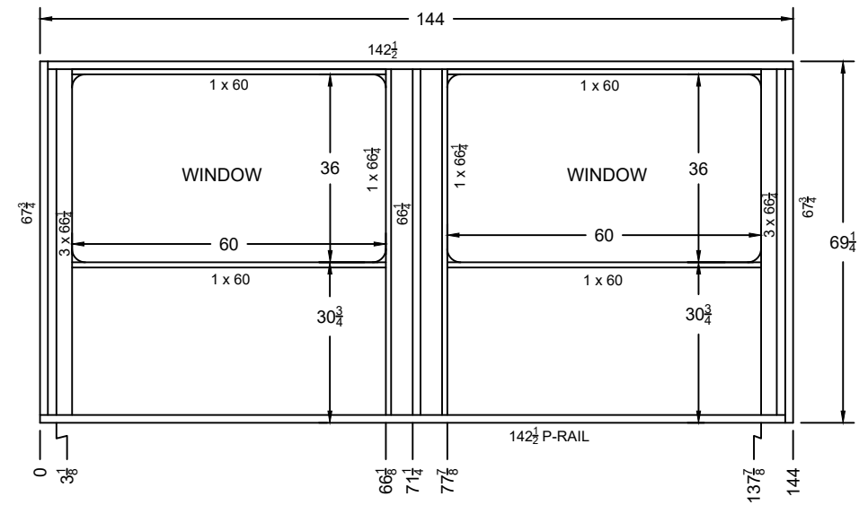
DINETTE PLUG WALL
