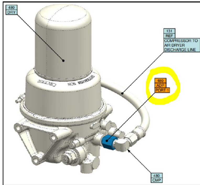
Fig. 2 Adapter
