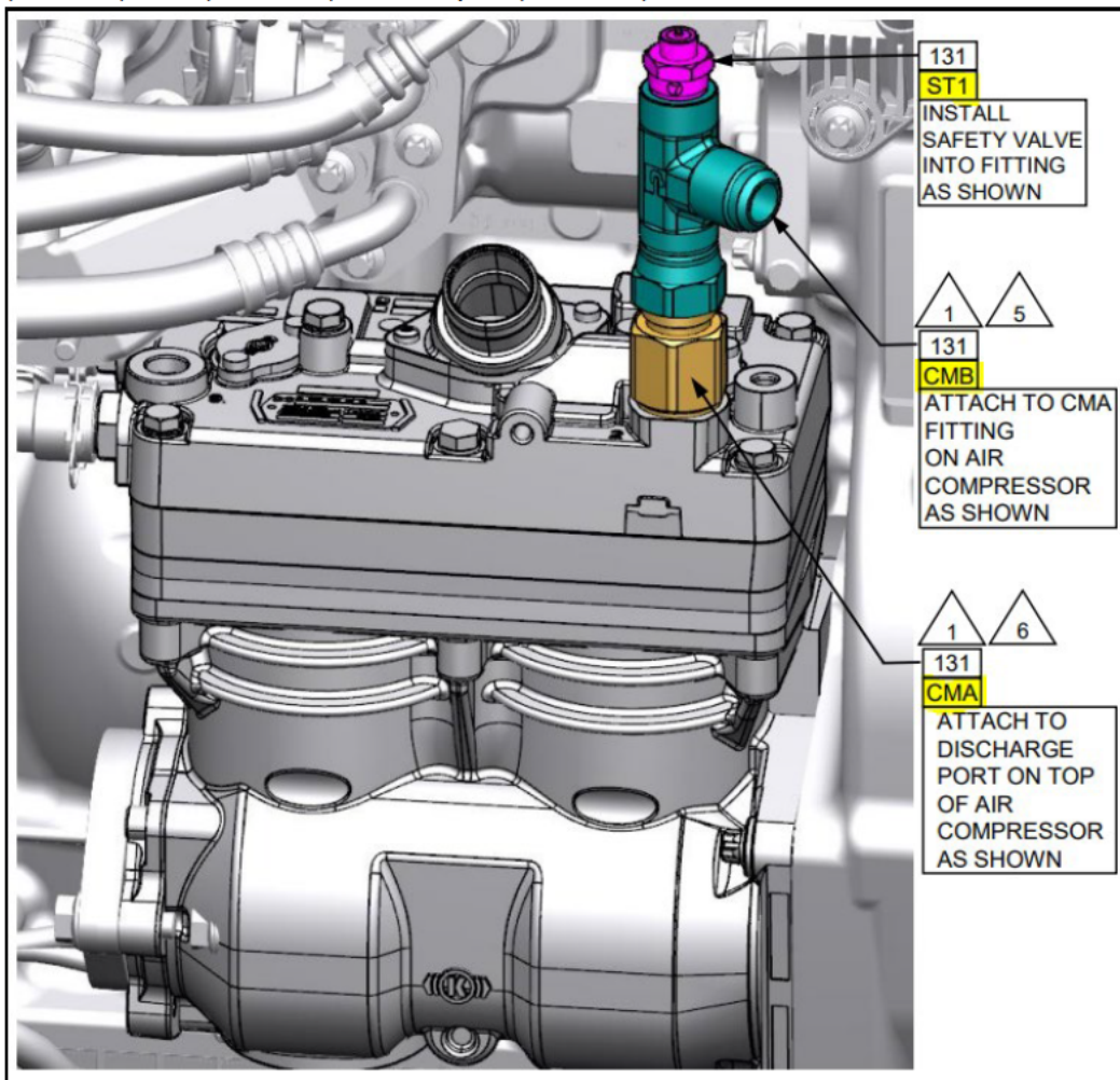
Fig. 1 Safety Valve, Fitting and Discharge Port
