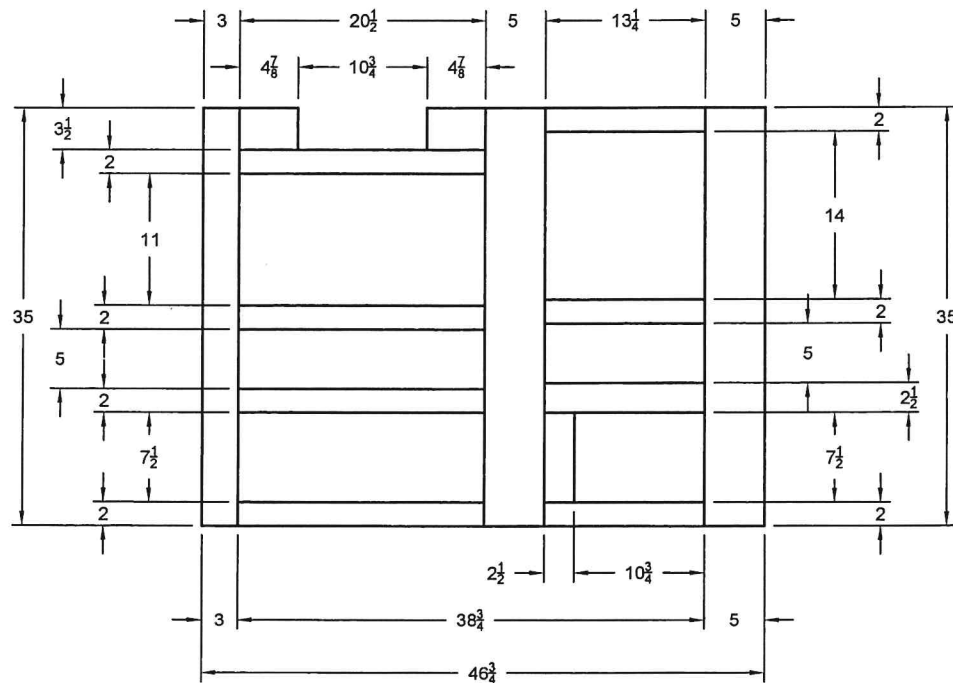
Face Frame Viewed From The Backside
