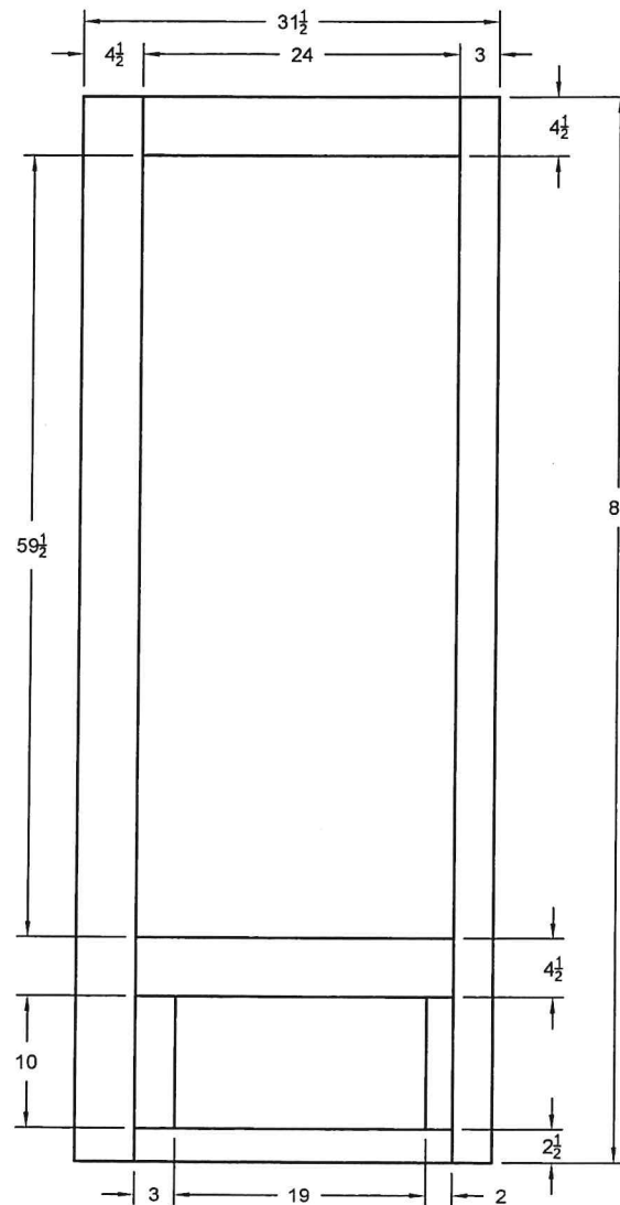
Face Frame Viewed From The Backside
