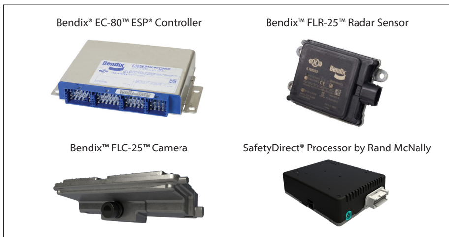
Figure 3 – System Components
