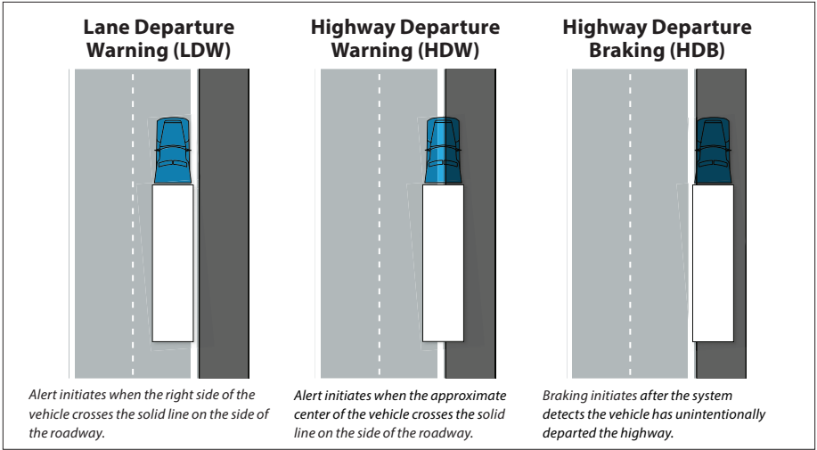
Figure 24 – LDW, HDW, and HDB
