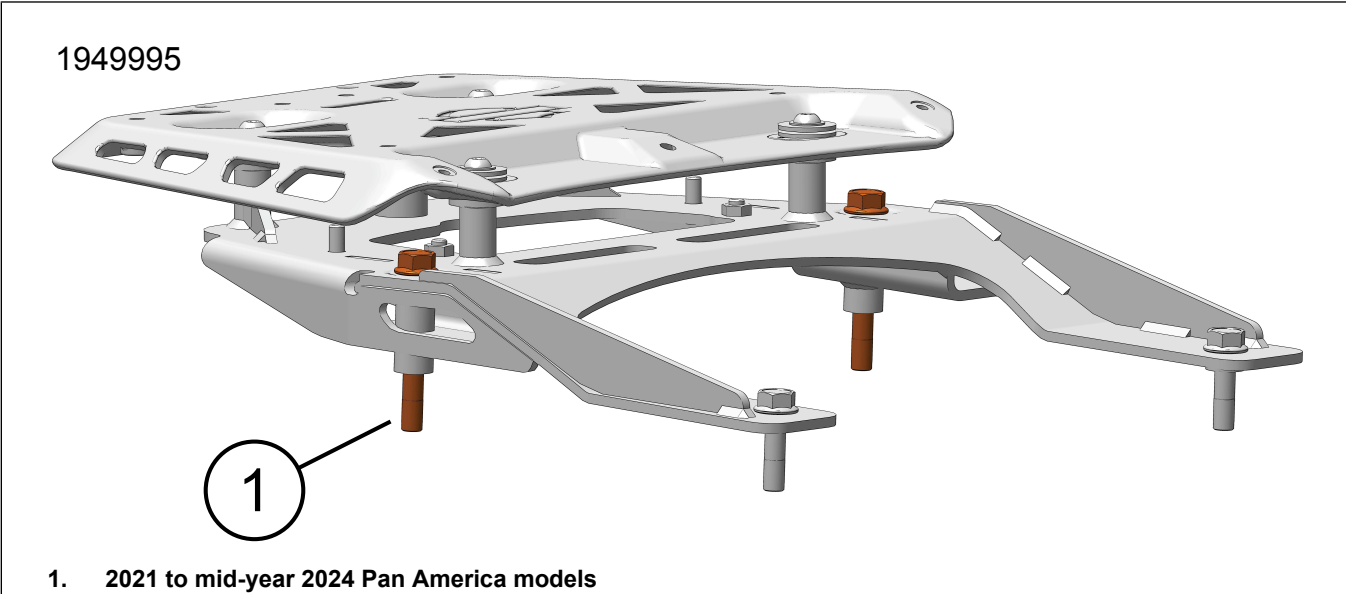
Figure 2. Kit No. 53000800, Screws Insert from Top and Thread Into Rear Frame Spools
