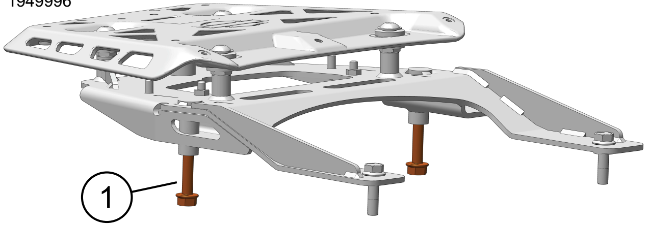
Figure 3. Kit No. 53000800A, Screws Insert from Bottom and Thread Into Mounting Bracket Spools
