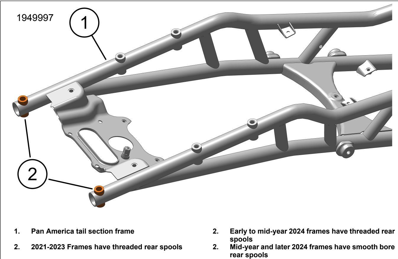
Figure 1. Tail Section Frame Rear Spools
