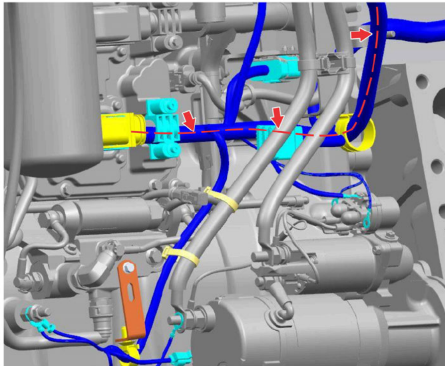
Fig. 40, Engine Overlay Routing Path (Cummins X15)
