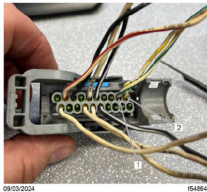
Fig. 69, Eaton Endurant ECU Connector J1939 Pin Locations
