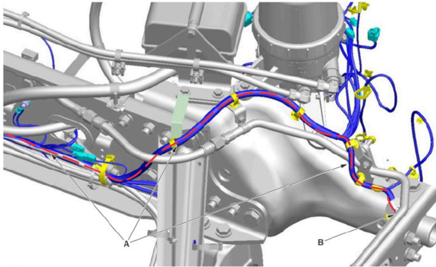
Fig. 74, Routing Path of ACC Extension Harness A66-37418-000 Along Left Frame Rail
