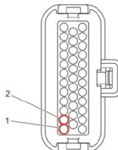
Fig. 96, Optimax 35-Pin Connector J1939 Pin Locations
