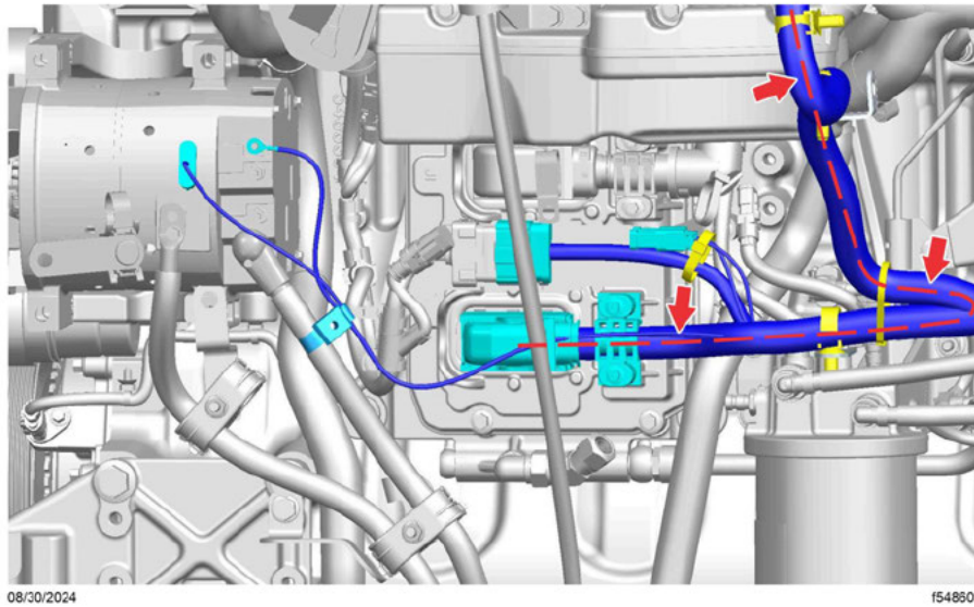
Fig. 38, Engine Overlay Routing Path (Cummins X12)
