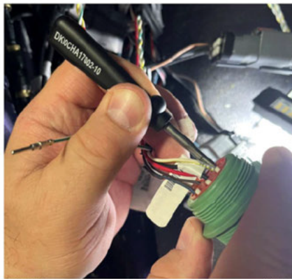
Fig. 18, Releasing and Removing J1939 Wires From the Diagnostic Connector Using Terminal Tool DK10CHA17002-10
