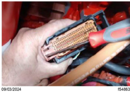
Fig. 61, Cummins ECM Connector Terminal Lock Removal
