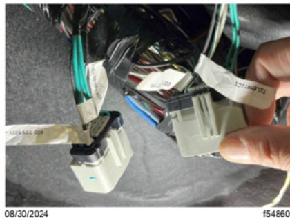
Fig. 36, Typical RP1226 Connectors (RP1226 1 and TGS RP1226 Shown)
