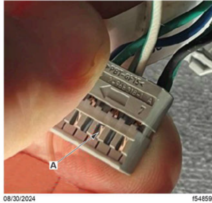
Fig. 24, CGW Connector Pinout: CAV 4 J1939+ (Y) And CAV 9 J1939- (DKG)
