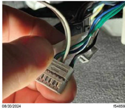
Fig. 23, Gray Connector Removed from Main CGW Connector Housing
