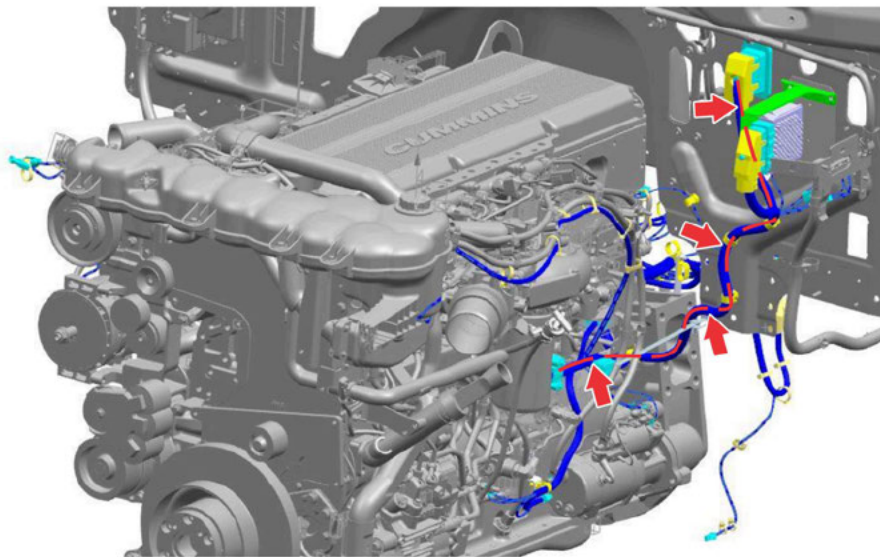
Fig. 41, Engine Overlay Routing Path from ECM to Bulkhead Connector BHA (Cummins X15)
