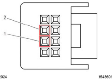
Fig. 30, Wabco Display Connector J1939 Pin Locations
