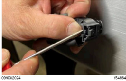
Fig. 77, Removing Outer Shell From Forward Radar Connector
