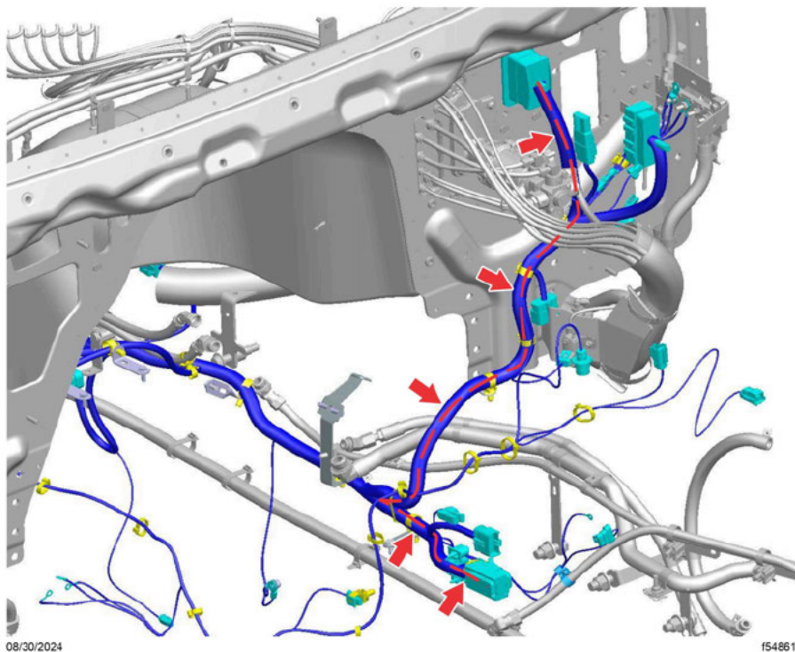
Fig. 38, Engine Overlay Routing Path (Cummins X12)
