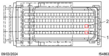
Fig. 62, Cummins ECM Connector J1939 Pin Locations
