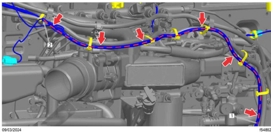
1. To connection with the engine overlay 2. To connection engine harness fan harness connector Fig. 56, Routing Path of EVIS-Fan Extension Harness A66-37416-000
