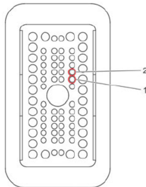
Fig. 43, Bulkhead Connector BHA J1939 Pinout Locations
