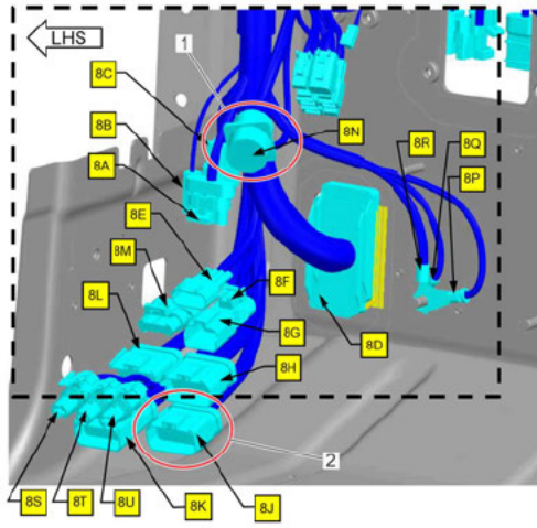
1. DL_DASH_O_JCT_DIGN_9P_1C 2. DASH_H_FLR_LH_CBL_4B Fig. 20, Diagnostic Connector and Floor Harness Connector Locations
