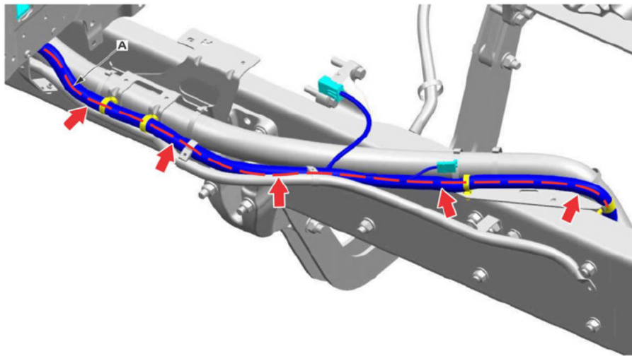
Fig. 70, Chassis Overlay Harness Routing Engine/Firewall Area
