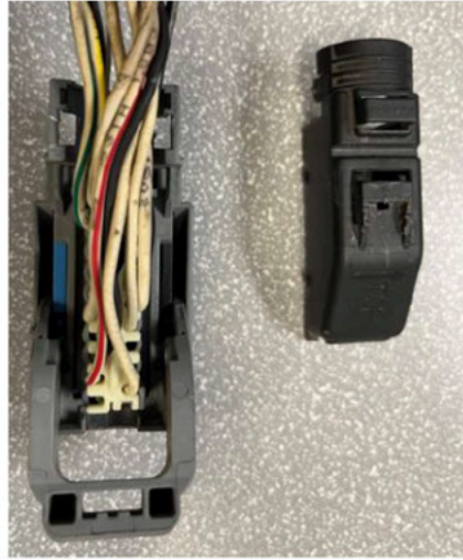
Fig. 66, Removing Backshell from Eaton Endurant Connector
