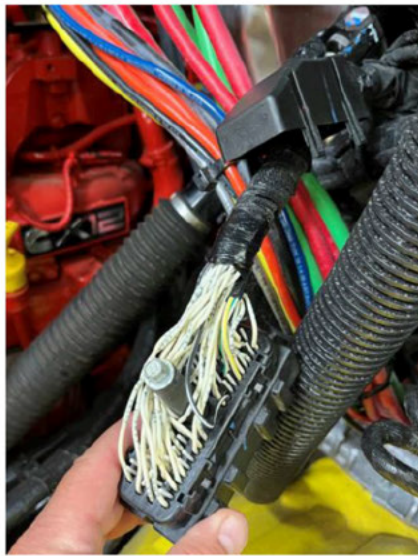
Fig. 48, Allison ECU Connector Backshell Removed
