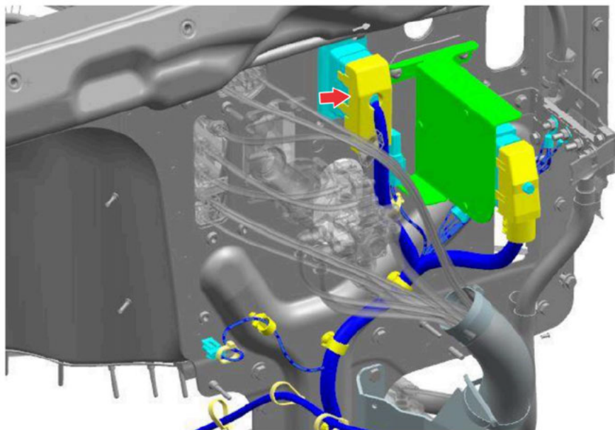
Fig. 42, Bulkhead Connector BHA
