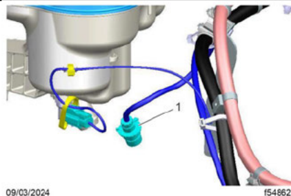
1. Fan Connector from the Engine Harness
