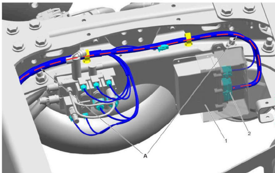
Fig. 94, Routing Optimax Extension Harness A66-37422-000
