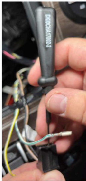
Fig. 31, Removing J1939 Wires from Wabco Display Connector Using Terminal Tool DK10CHA17002-2
