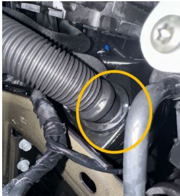
Figure 1. Filler hose not fitted correctly.
