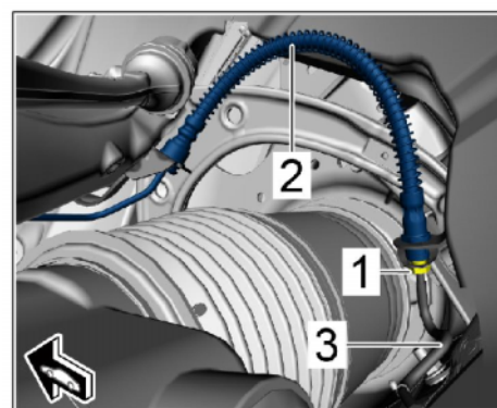
Front brake hose on vehicle-side brake line
