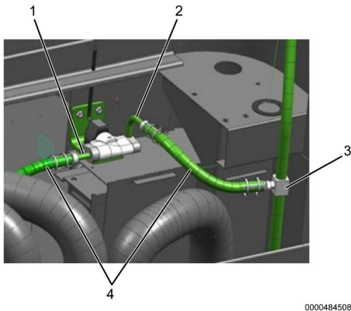
Figure 38. Dash Mounted A/C System Hose Location
