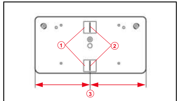
Figure 31. Front License Plate Mounting Bracket
