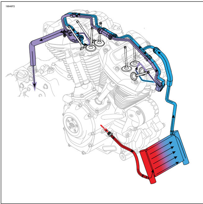
Figure 2. Air/Oil-Cooled
