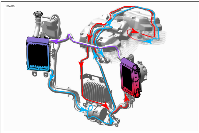
Figure 3. Twin-Cooled
