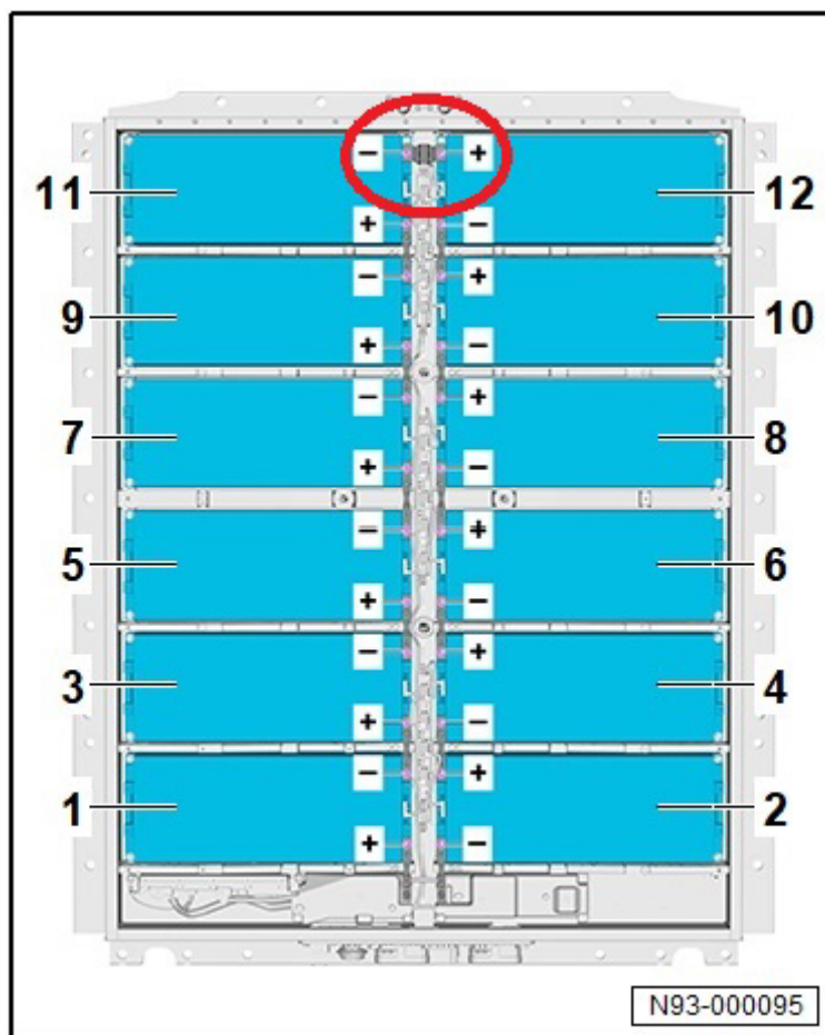
Figure 2. High-voltage connector opposite coolant connection.
