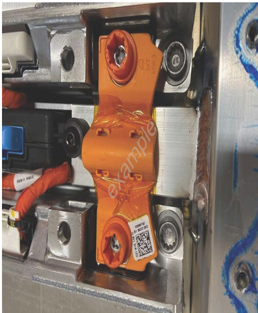
Figure 1: Film/adhesive tape wrapped around high-voltage connector (example).
