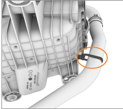
Image 1 Location of the retaining clip. Image shows correct cable tie with an edge clip (1)
