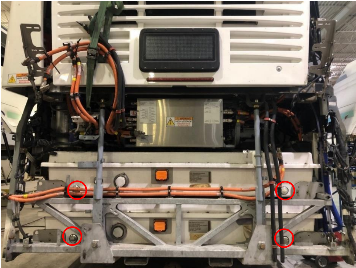
Figure 2: Rear ESS Layout and rear drain locations
