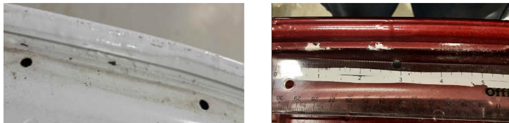
Hem Flange Area Examples (Fig. 2)
