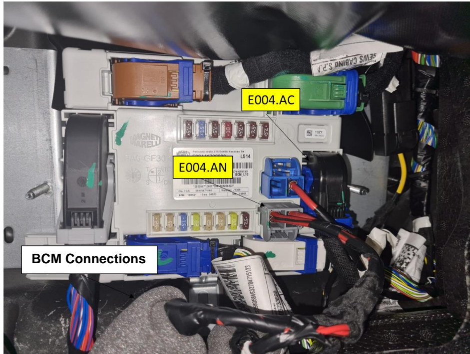
BCM Connection Locations for E004.AN and E004.AC
