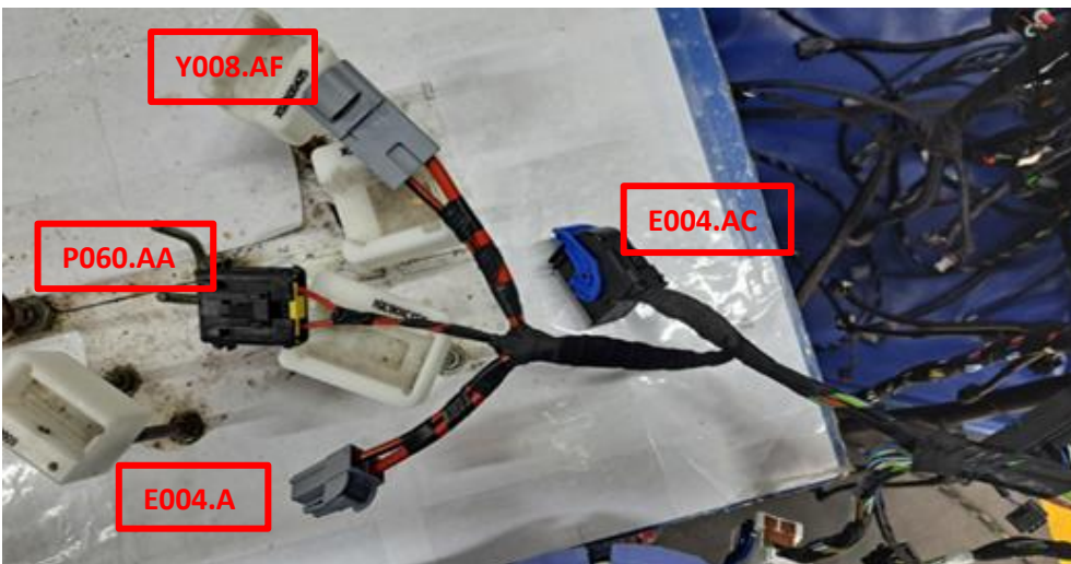
Front Wiring Harness Replacement: Configured with 2 additional connectors and 1 fuse holder
