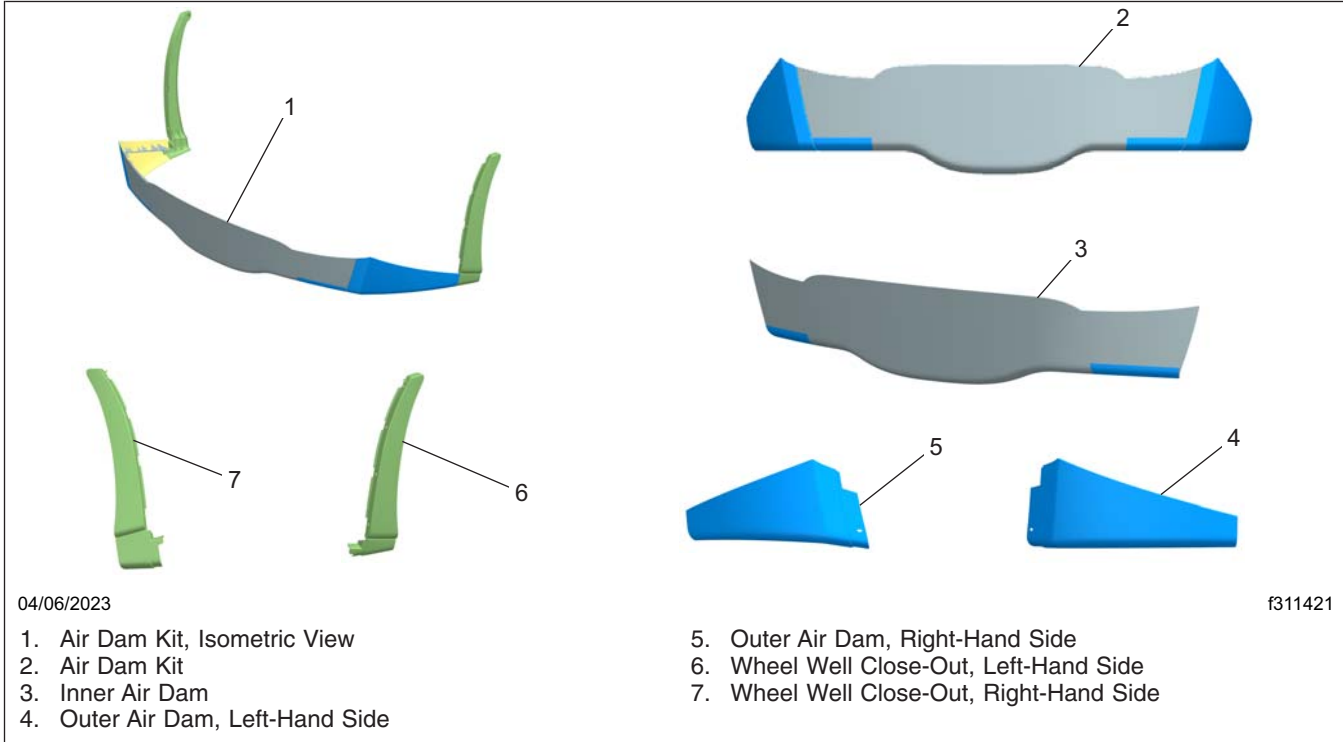
Fig. 2, 6-4-6 Air Dam Parts
