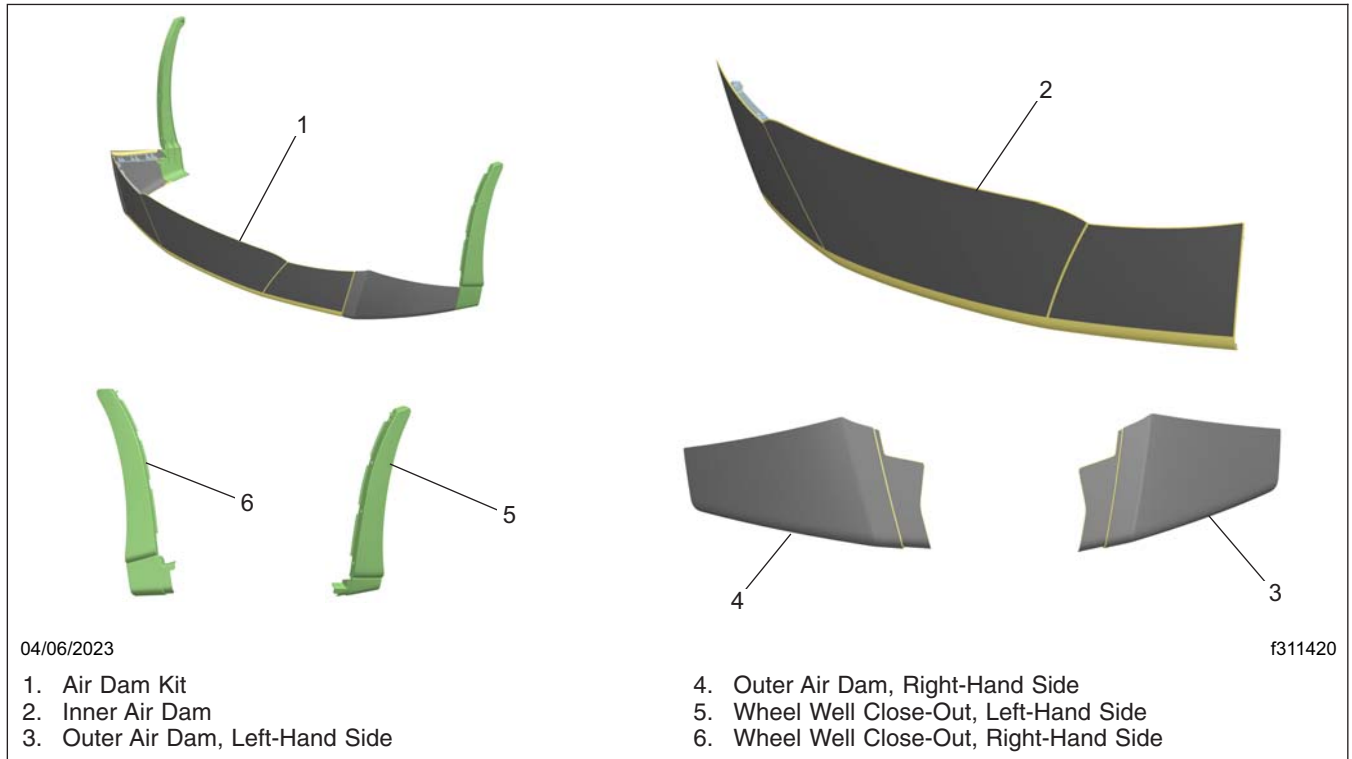
Fig. 1, 4-4-4 Air Dam Parts
