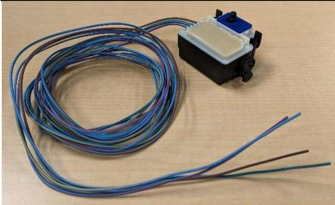
Figure 1. The Locking Actuator, as received as a spare part.
