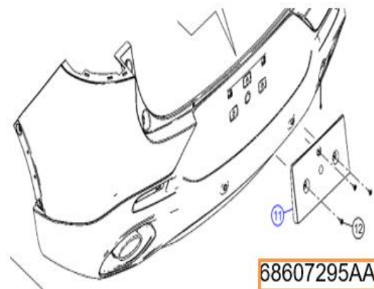
Plate Bracket and Screws
