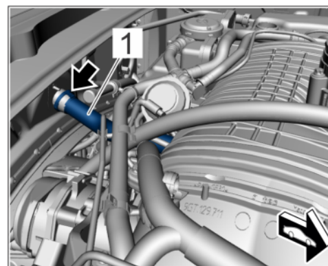
Oil filler pipe
