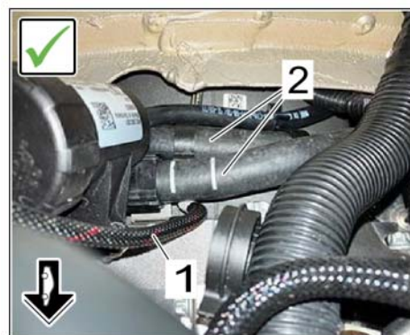
New positioning of control line for exhaust flaps
