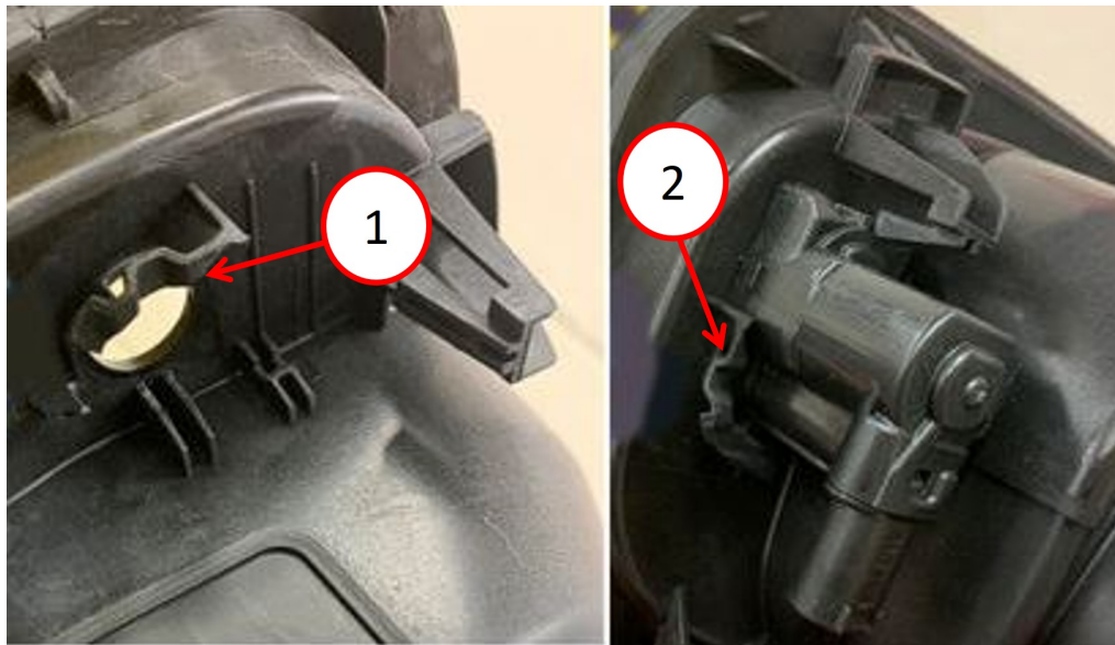
Fig. 1 Fuel Filler Door Housings
