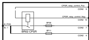
15/49 ENGINE JUNCTION BOX
