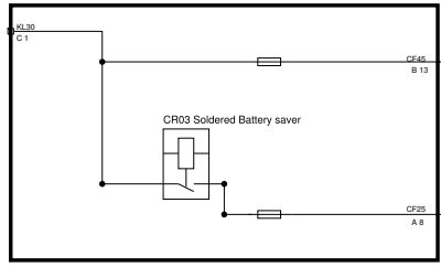
15/50 CENTRAL JUNCTION BOX
