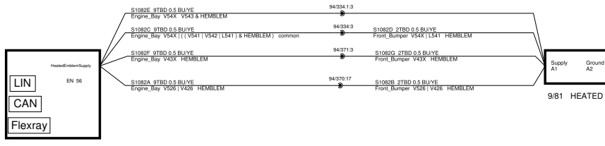
4/56 CENTRAL ELECTRONIC MODULE CEM
