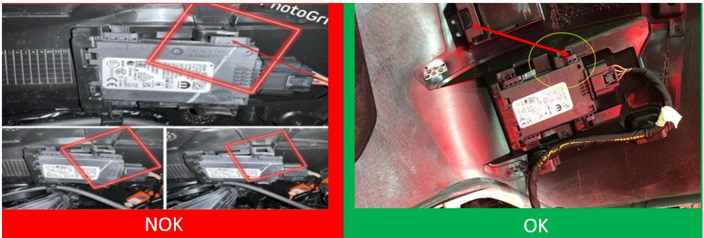
Fig 1 MRR installation. Module mounting tab engagement.
