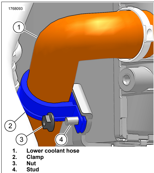
Figure 2. Lower Coolant Hose Clamp
