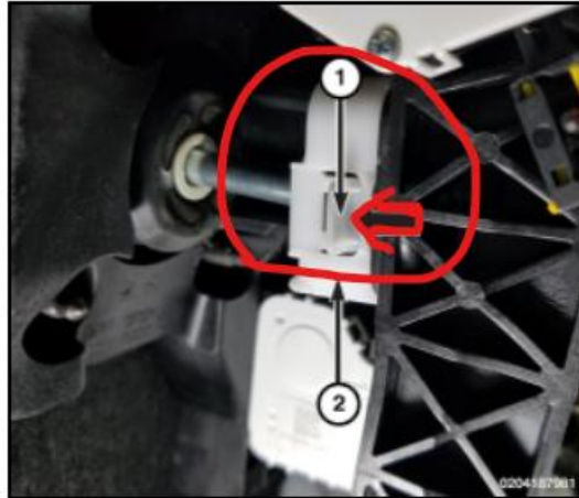
Clips engaged
