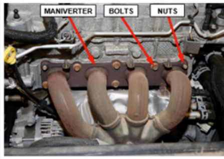
Maniverter to Engine
