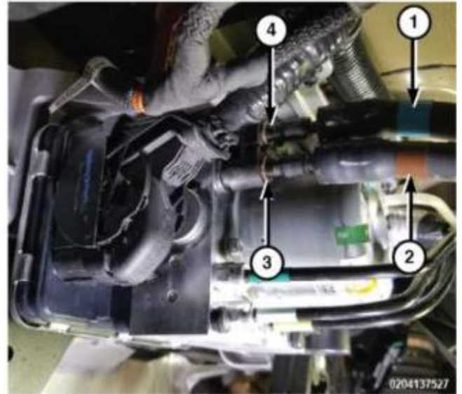
Proper removal of the intake and outlet line assemblies
