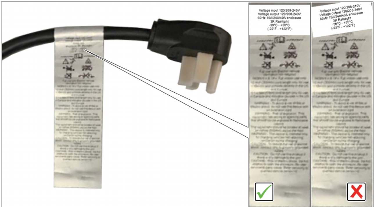
Bonding position
