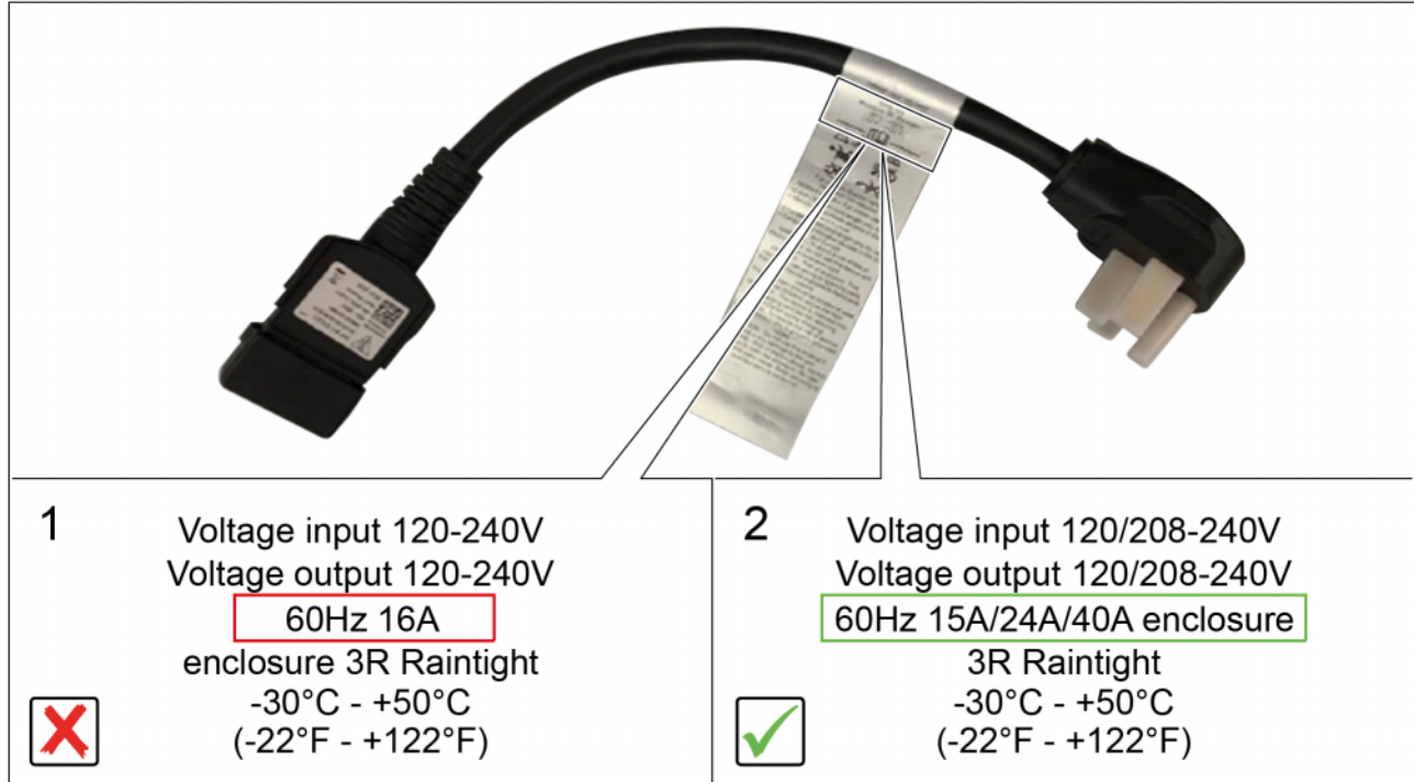
NEMA infrastructure charging cable label
