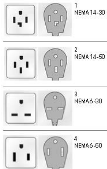
Overview of NEMA plug contacts
