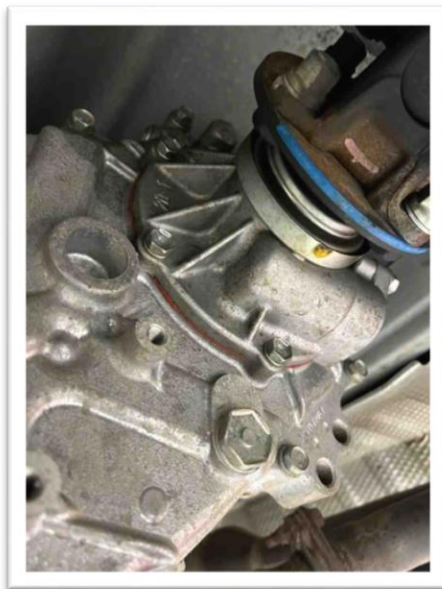
Figure 1 Rear Output Shaft Seal Leak
