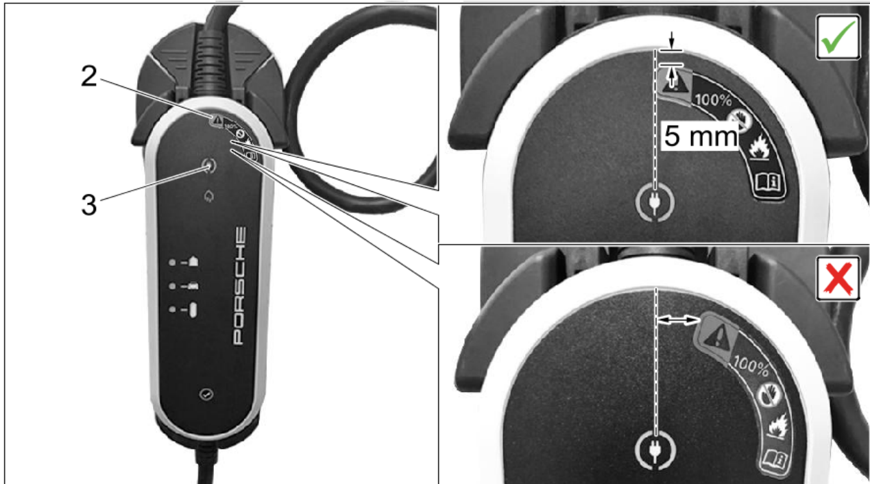
Bonding position
