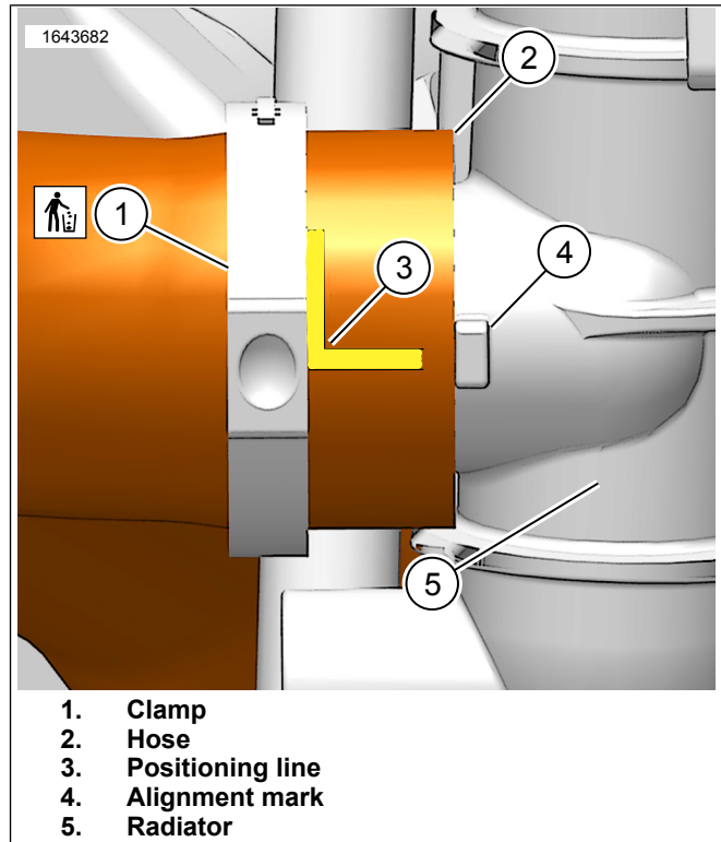
Figure 3. Lower Coolant Hose to Radiator
