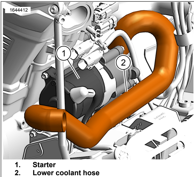
Figure 1. Lower Coolant Hose Routing
