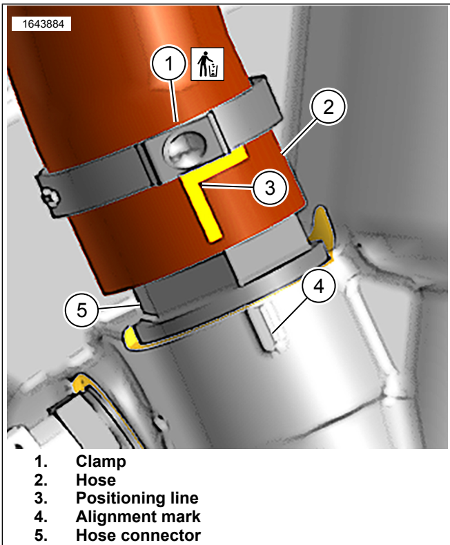
Figure 2. Lower Coolant Hose to Engine
